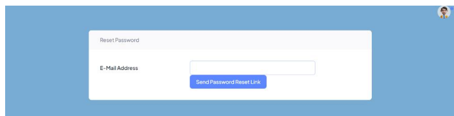
Gambar 7. Forgot Password
